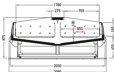
LDLH-12 BCA class M1
