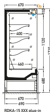
RDKA-15 XXX plug-in
