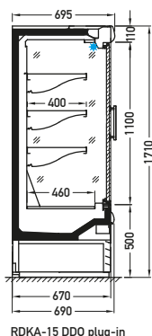
RDKA-15 DDO plug-in
